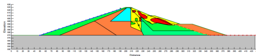
Fig. 11. Model dam using on cross-section +85m
