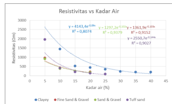
Fig. 6. Variation of soil resistivity value with water content
