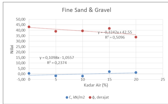
Fig. 7. Variation of c and φ value with different water content on Fine Sand & Gravel
