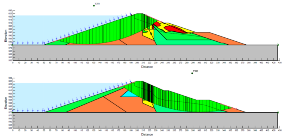
Fig. 14. Stability analysis on +85m after applying seismic load for a return period of 50 years
