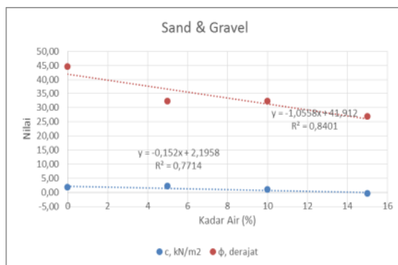
Fig. 8. Variation of c and φ value with different water content on Sand & Gravel
