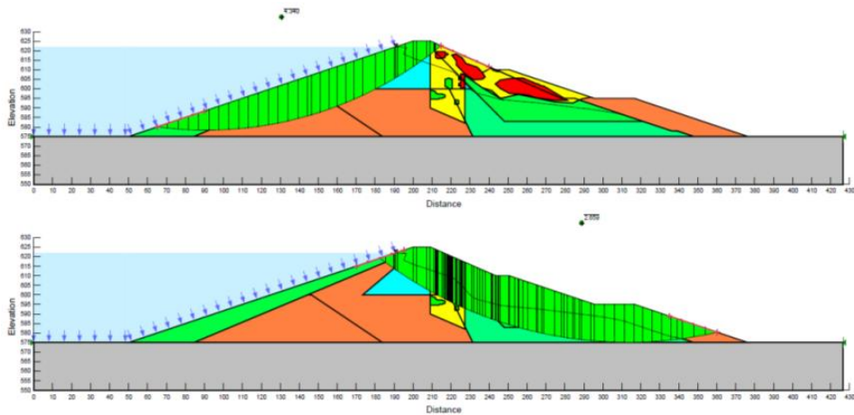
Fig. 13. Stability analysis results on cross-section +85m before applying Seismic load
