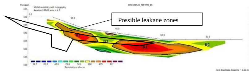
Fig. 4. Soil resistivity imaging along cross-section line 85m
