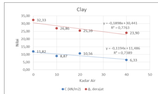
Fig. 10. Variation of c and φ value with different water content on Clay
