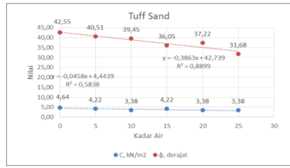
Fig. 9. Variation of c and φ value with different water content on Tuff Sand
