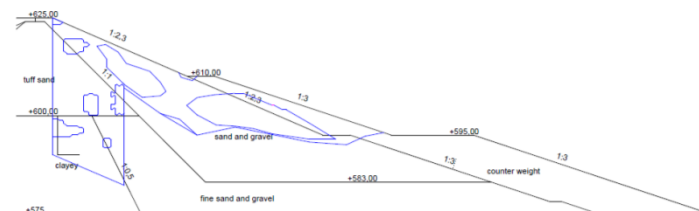
Fig. 5. Cross-section of model on line 85m
