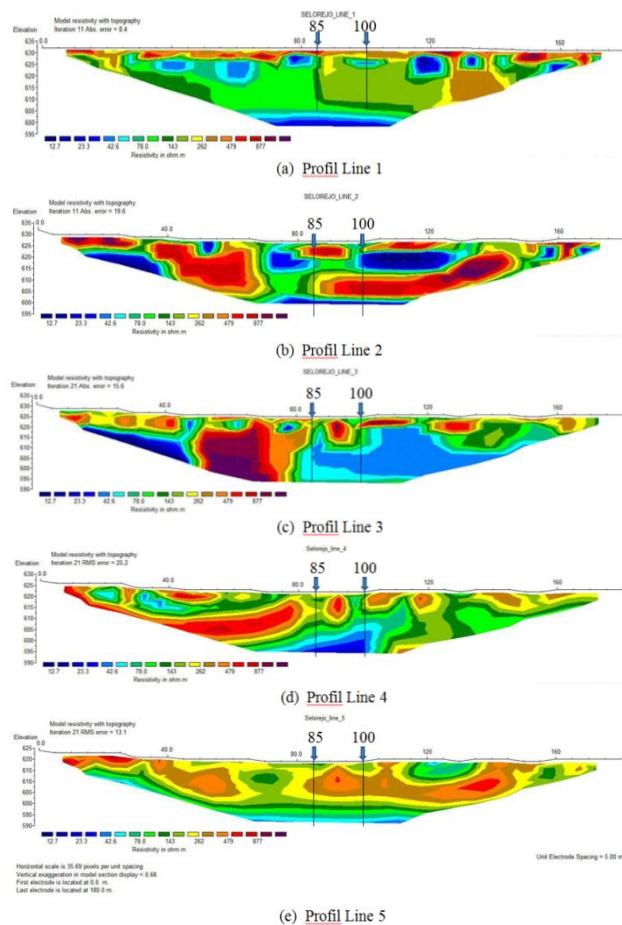
Fig. 3. Soil resistivity imaging along the body of the earth dam
