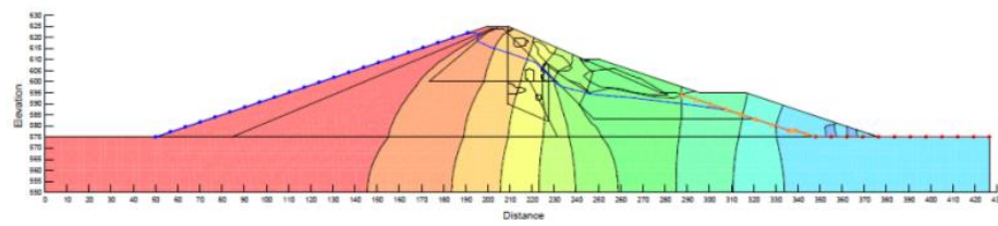
Fig. 12. Seepage analysis results on cross-section +85m
