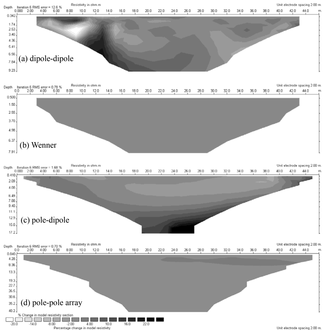
Fig. 5 Percentage change of inverted resistivity between two repeated measurements for (a) dipole-dipole; (b) Wenner; (c) pole-dipole; and (d) pole-pole array, respectively
