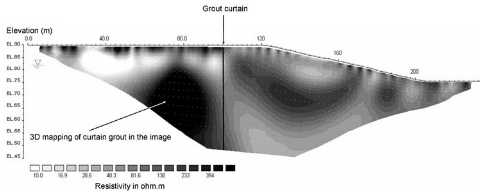
Fig. 6 Inverted resistivity cross-section for Line C at the left abutment
