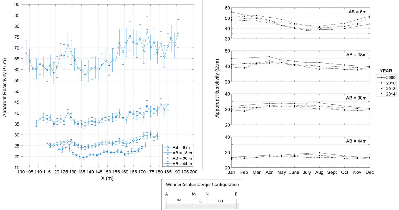
Fig. 3. Raw Wenner-Schlumberger apparent resistivity ( \Omega\cdot\text{m} ) data acquired with the electrode line situated on the land side. Left: Selected apparent resistivity profiles for each monthly acquisition in 2014; Right: Mean apparent resistivity for each selected profile and monthly acquisition for years 2009, 2010, 2013 and 2014.
