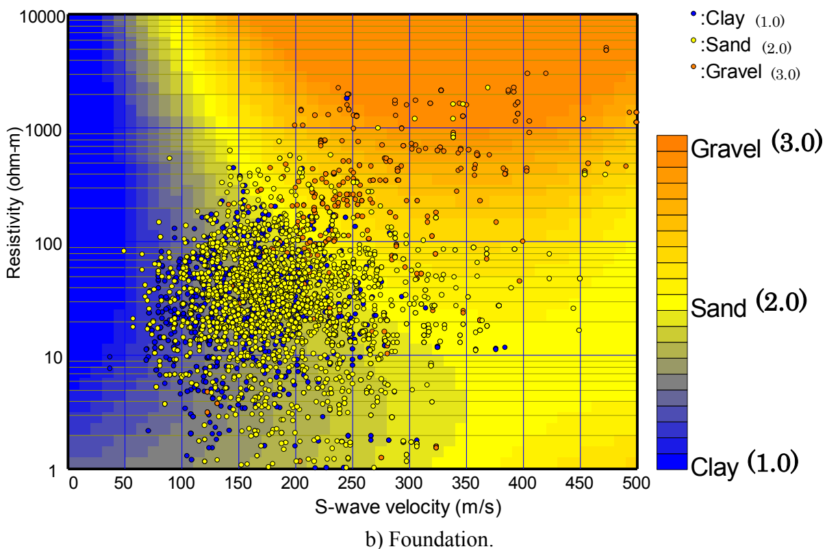
Figure 2: Distribution of soil parameter S as a function of S-wave velocity and resistivity calculated from a polynomial approximation.
