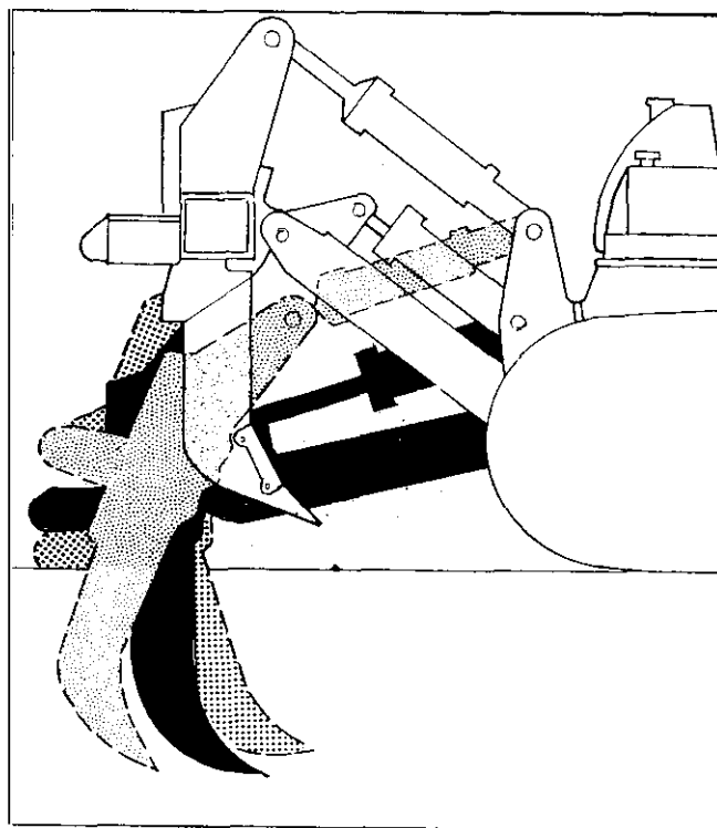
Adjustable parallelogram ripper combines radial and parallelogram traits, with varying tip-to-ground angle as the ripper penetrates.
