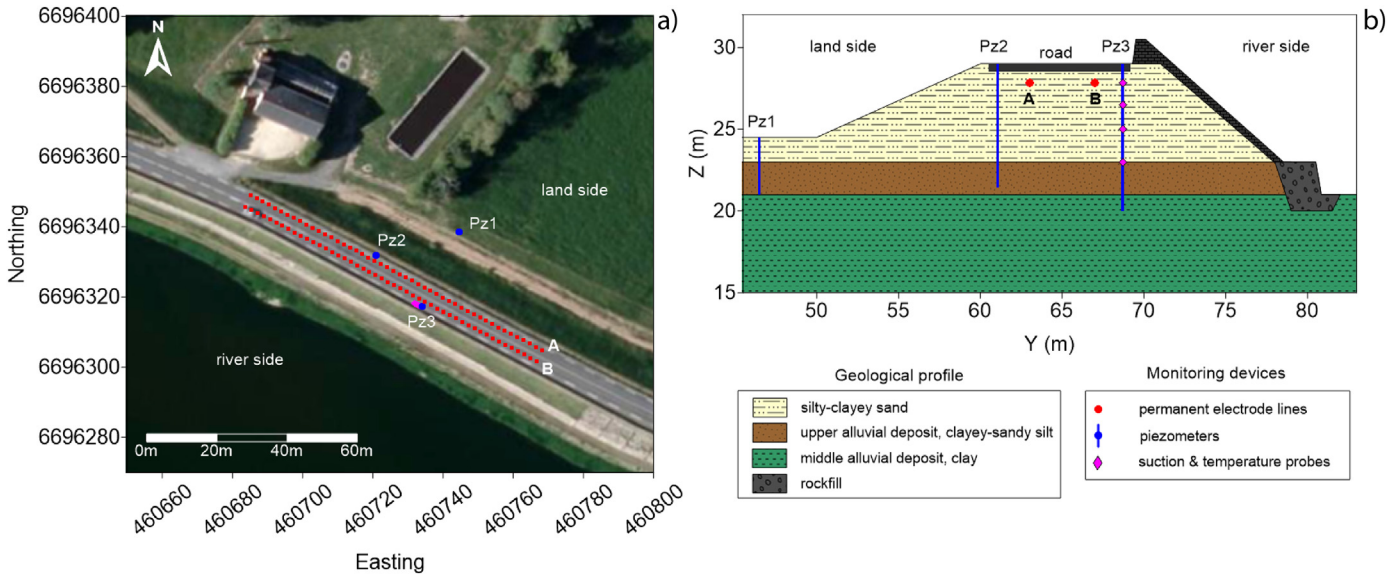
Fig. 1. a) Satellite view of the site (in Lambert 93 coordinates, ©Google Earth) and b) Geological cross-section of the Loire river levee and natural foundation with the permanently installed ERT lines and additional monitoring devices. The thick dark grey parts represent the road structure and the masonry revetment on the crest and the river side slope respectively.
