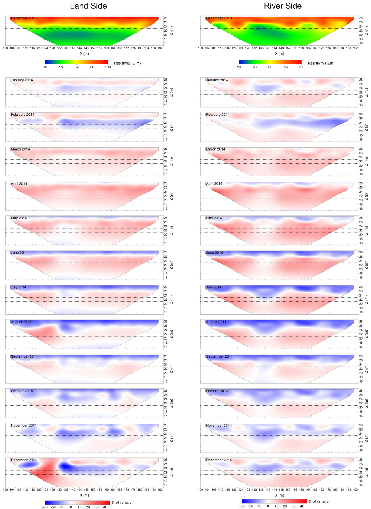
Fig. 4. 2D inverted resistivity tomographies for the reference date of December 2013 (top sections) and percentage resistivity change sections from "cascade" inversions for a) the land side and b) the river side. The dotted lines represent the top of each alluvial layers estimated according the geotechnical data (Fig. 1).
