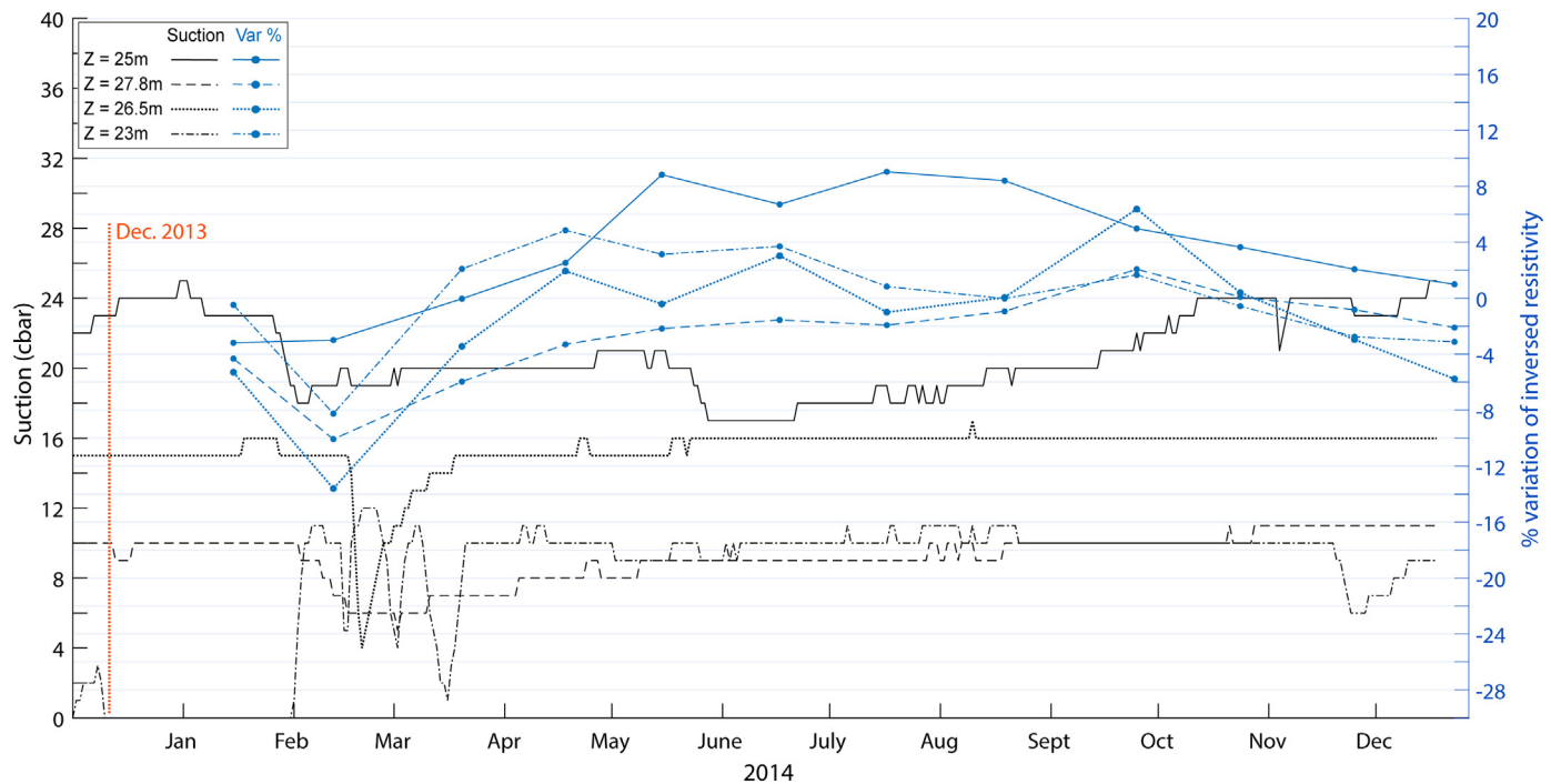
Fig. 8. Comparison of time-series graphs of suction direct measurements within the levee body and time-series graphs showing average percentage resistivity changes for temperature-compensated resistivities of the river side of the levee, over the year 2014 and at four depths.
