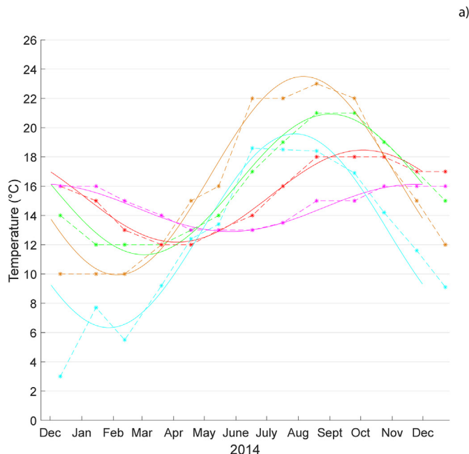
Fig. 2. a) Observed and modelled soil temperatures for surface and subsurface probes at five depths; b) Modelled soil temperature at each resistivity inversion depth for the reference date, December 2013, and each month of year 2014.
