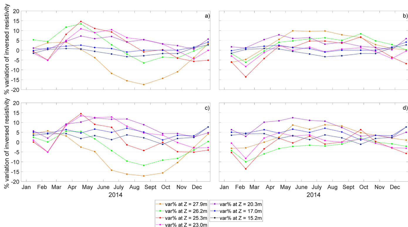
Fig. 6. Time-series graphs showing average percentage resistivity changes with time at seven different elevations in the levee body, for the land (a. and b.) and the river (c. and d.) sides of the levee, and for non-compensated (a. and c.) and temperature-compensated (b. and d.) resistivities.
