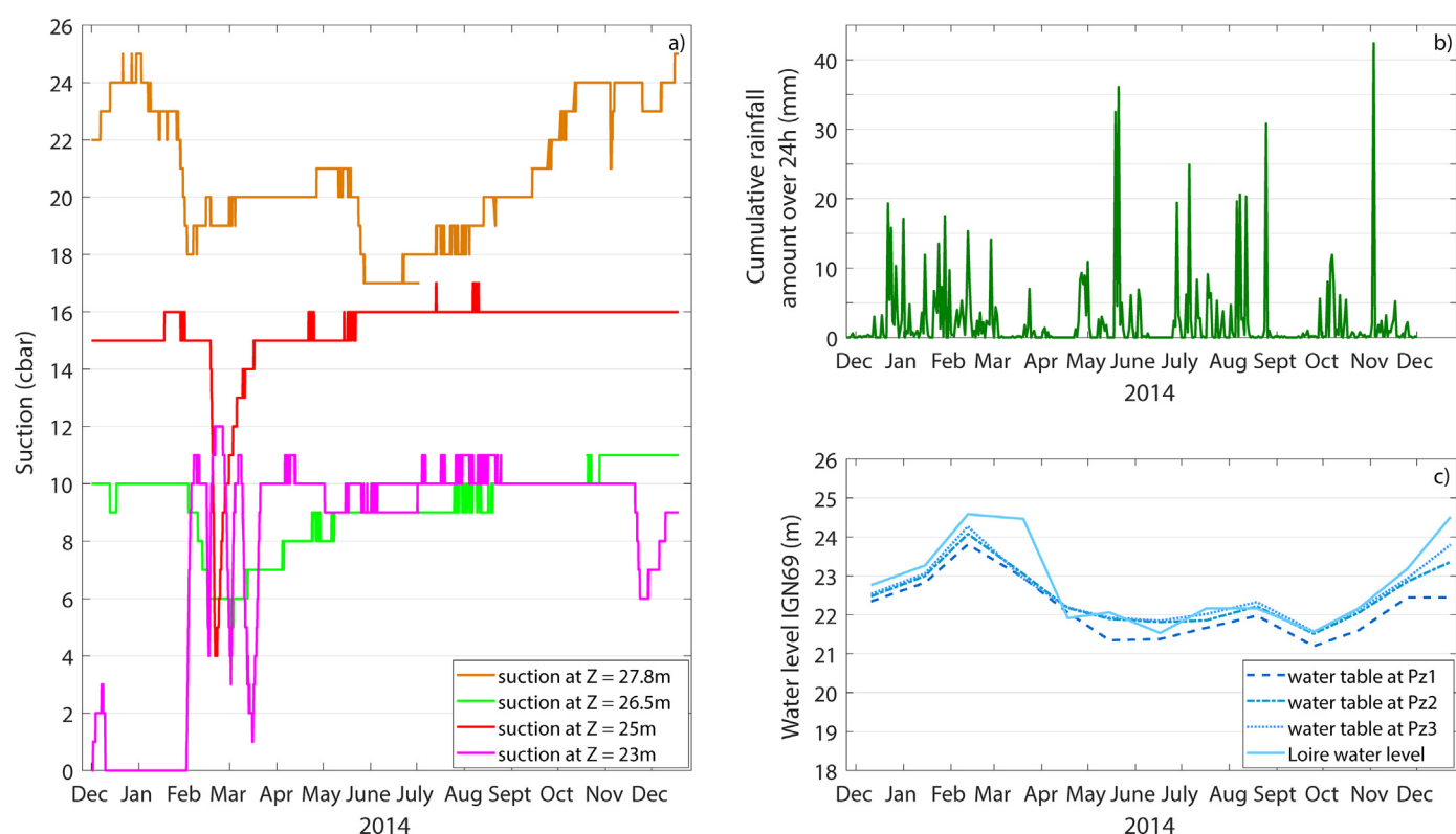
Fig. 7. Time-series graphs of direct observations over the year 2014 for: a) Suction at four depths within the levee body; b) Daily cumulative rainfall recording (MeteoFrance ©) and c) Monthly water table levels at piezometers Pz1 through Pz3 (Fig. 1) and monthly measured level of the Loire river.
