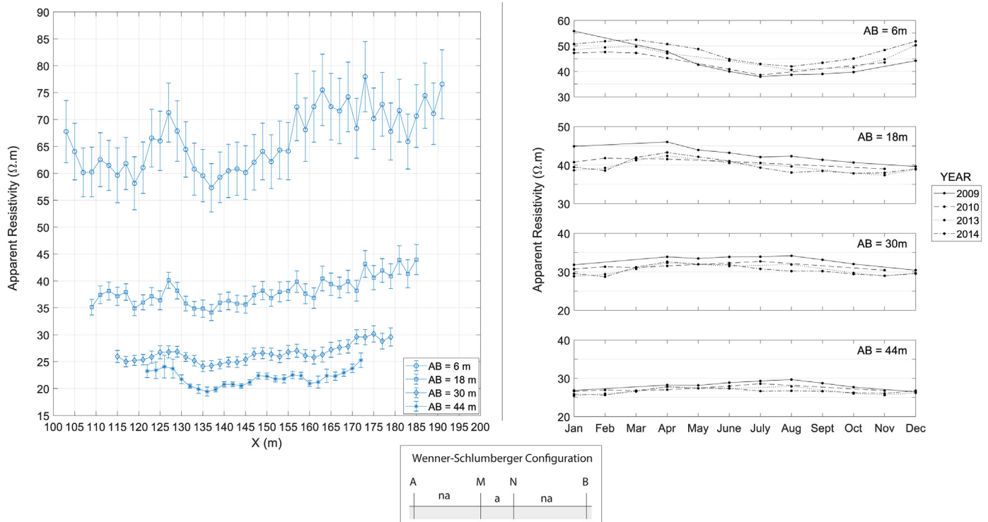
Fig. 3. Raw Wenner-Schlumberger apparent resistivity ( \Omega .m) data acquired with the electrode line situated on the land side. Left: Selected apparent resistivity profiles for each monthly acquisition in 2014; Right: Mean apparent resistivity for each selected profile and monthly acquisition for years 2009, 2010, 2013 and 2014.
