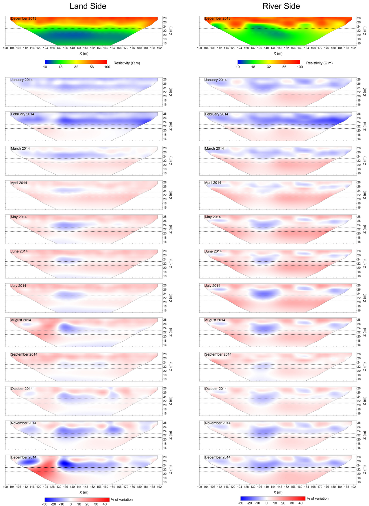
Fig. 5. 2D inverted resistivity tomography corrected of the modelled temperature (Fig. 2.b) for the reference date of December 2013 (top sections) and percentage resistivity change sections from "cascade" inversions for a) the land side, and b) the river side. The dotted lines represent the top of each alluvial layers estimated according the geotechnical data (Fig. 1).
