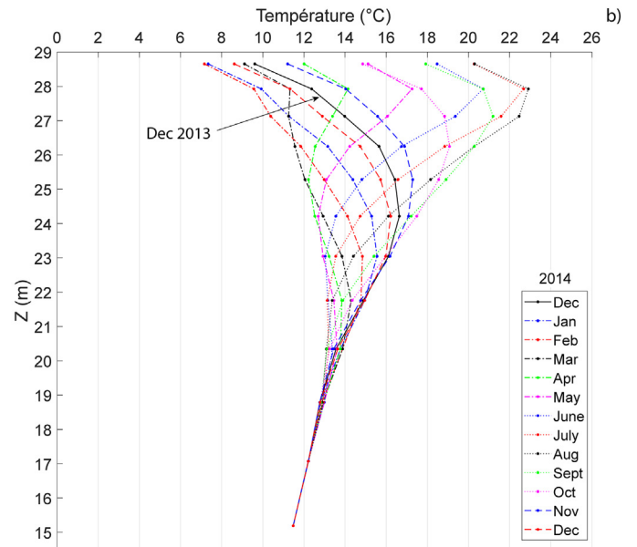
Fig. 2. a) Observed and modelled soil temperatures for surface and subsurface probes at five depths; b) Modelled soil temperature at each resistivity inversion depth for the reference date, December 2013, and each month of year 2014.
