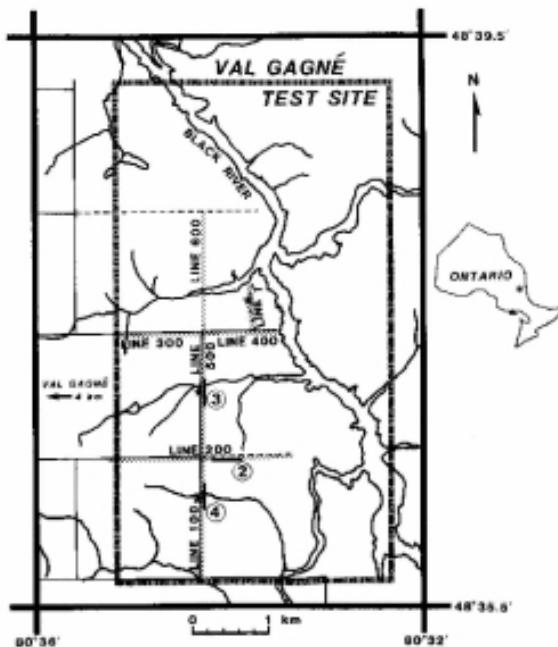
Figure 1. Map of the Val Gagne test site, indicating the location of seismic survey lines (hatched lines), drillholes (stars), and the sections shown in the following figures (solid lines related to circled numbers). Lines 100, 500, and 600 lie along the north-south baseline of the metric grid laid out for the test site; the east-west baseline is the southern limit of the site.
