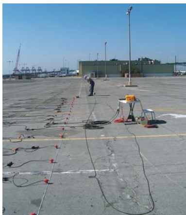
MASW Field Setup
