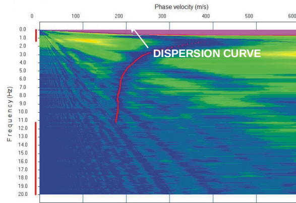
Dispersion Curve from Array Microtremor Measurements
