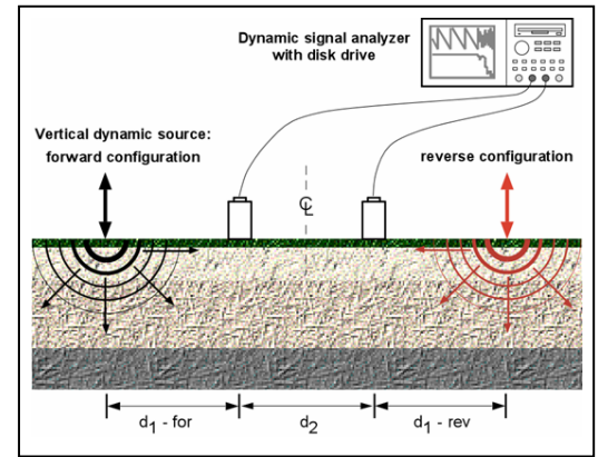
SASW Setup
